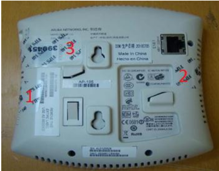
Figure 19 - Aruba AP-105 Tel placement bottom view
